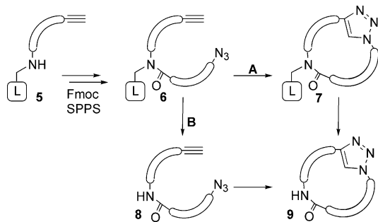
Scheme 1. Strategy for the combinatorial synthesis of triazole-containing cyclic peptides 9 .
