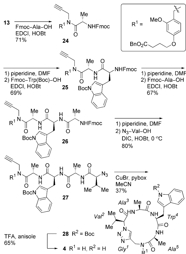
Scheme 5. Synthesis of the triazole analog 4 of segetalin B in solution from 13 .
