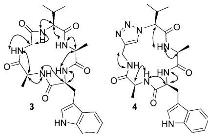
Figure 2. NOE correlations of cyclic peptide segetalin B ( 3 ) and its analog 4 .
