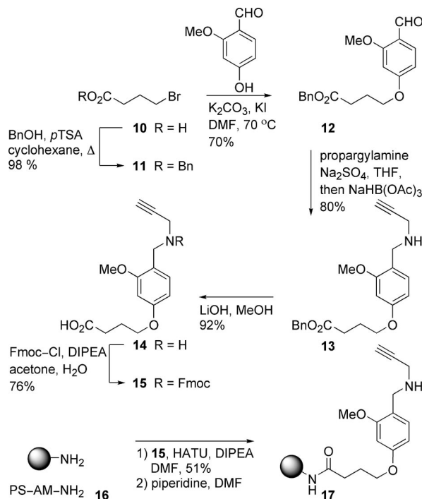
Scheme 2. Synthesis of the solution-phase linker 13 and the solid-phase linker 17 .
