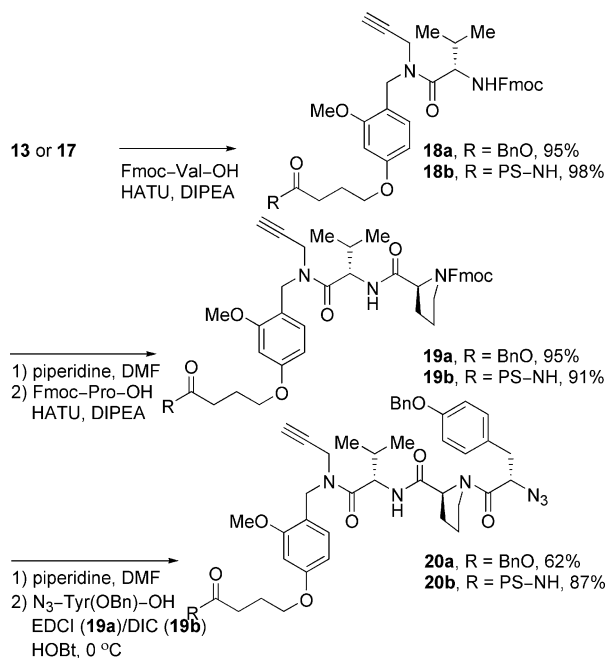
Scheme 3. Synthesis of the linear precursors in solution 20a from 13 and on the solid phase 20b from 17 .
