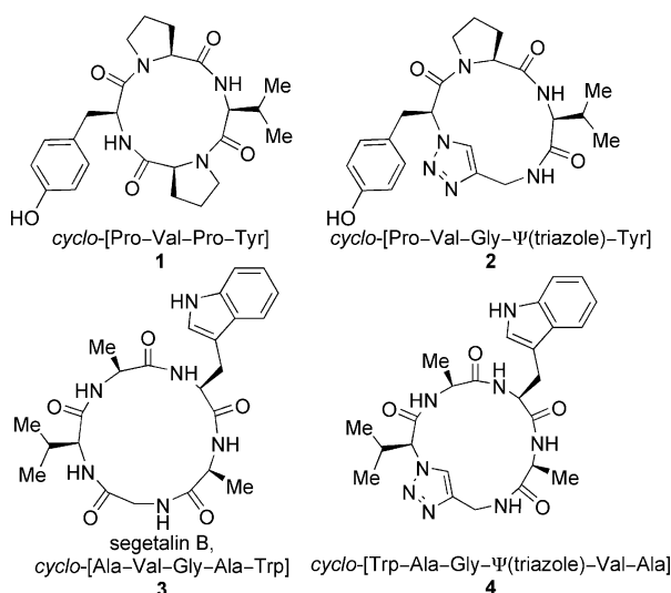
Figure 1. Cyclic peptides 1 and 3 and their triazole analogs 2 and 4 .
