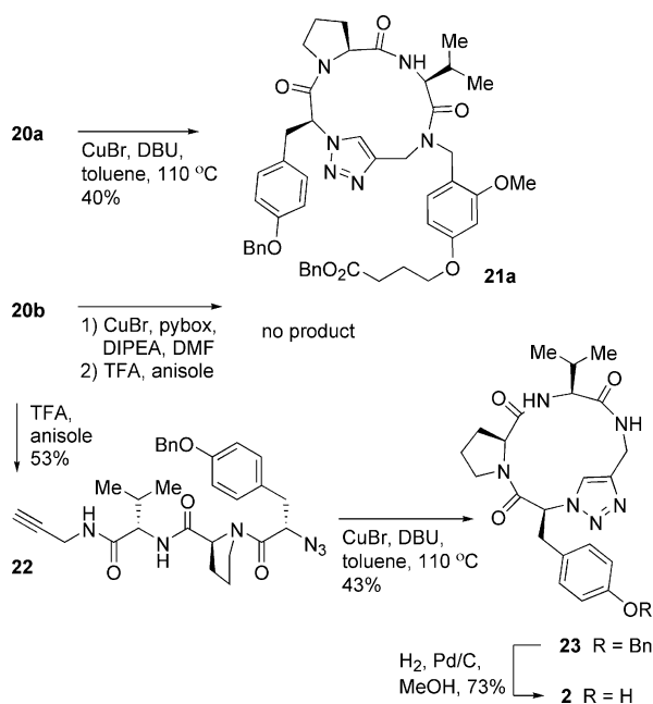
Scheme 4. Cyclization of the linear precursors 20a and 20b to afford the cyclic peptides 21a and 2 , respectively.
